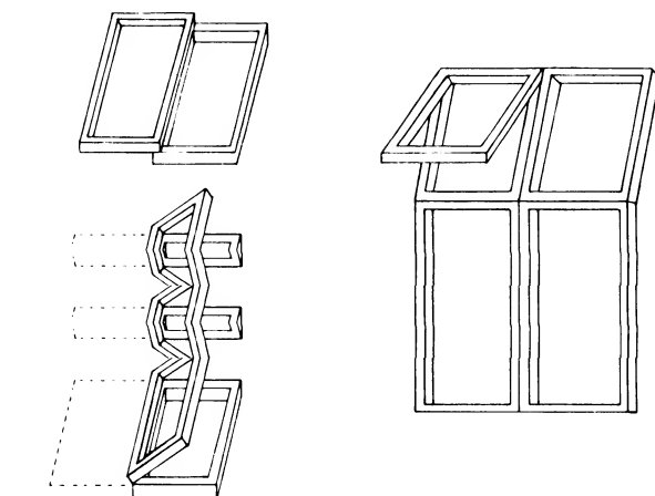
③ Sliding windows; escape
